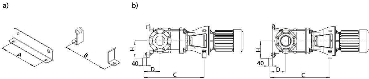
Fig. 75: a) Pump bracket b) Pump set
