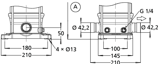
Fig. 5: Connections of Movitec VV, VSV
