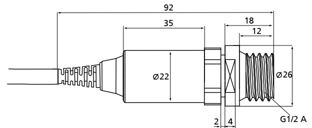
Fig. 9: Dimensions of sensor, measuring range 65 bar and above
