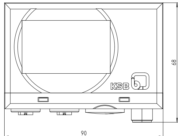
Fig. 10: Dimensions of the display unit
